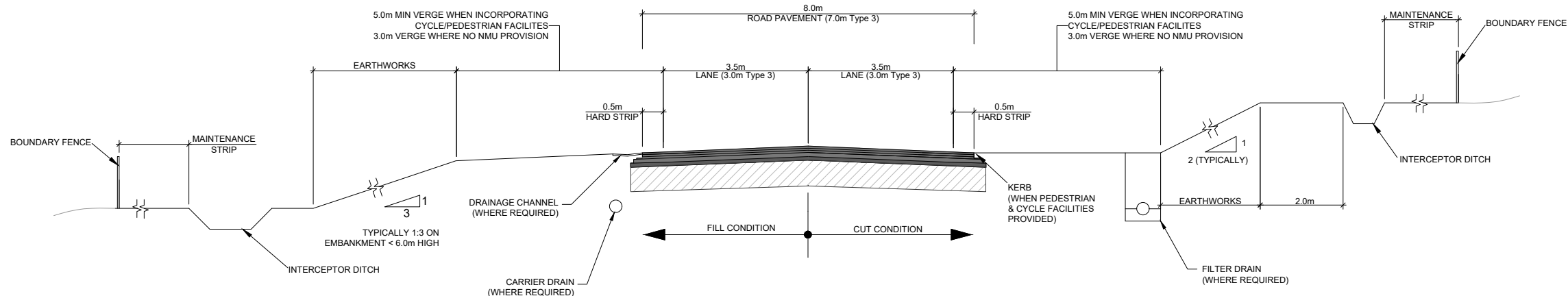
TYPE 2/3 SINGLE CARRIAGEWAY (S2)
