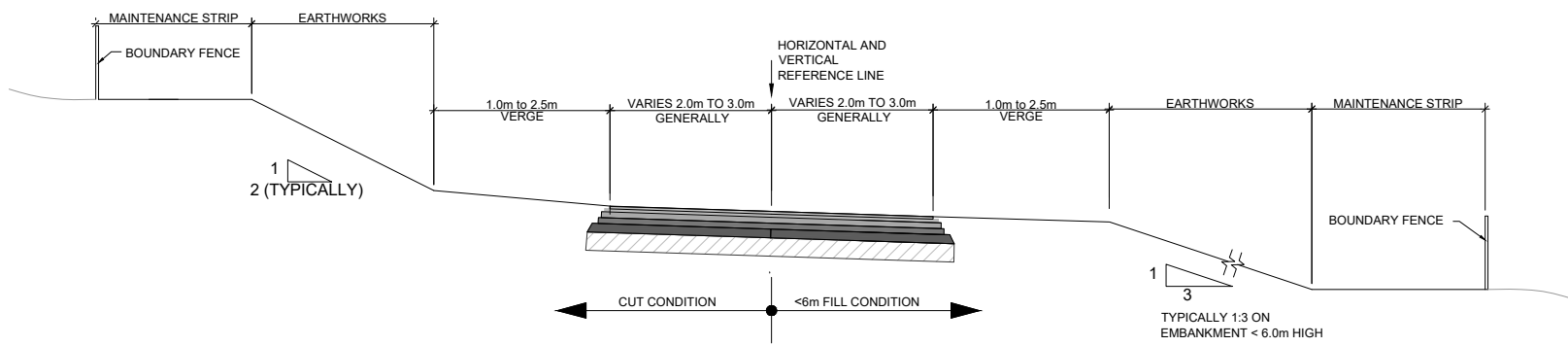
TYPICAL LOCAL ROAD CROSS SECTION
