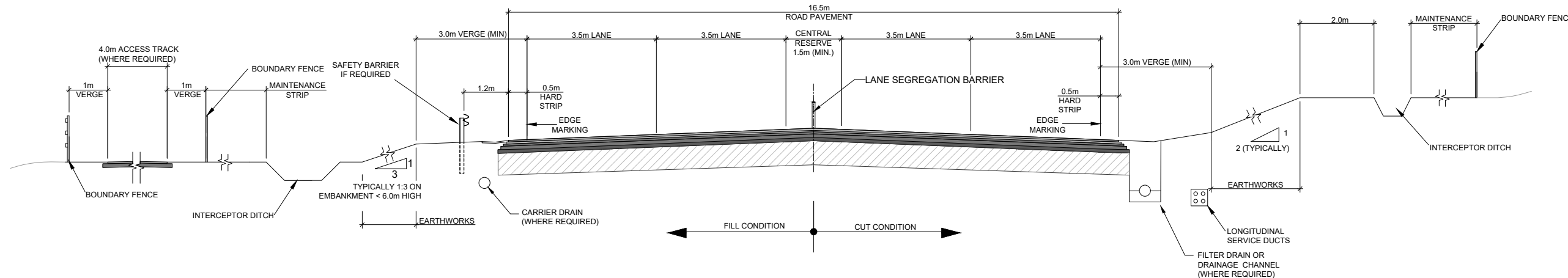
MAINLINE - TYPE 2 DUAL CARRIAGEWAY RURAL (D2AP)
